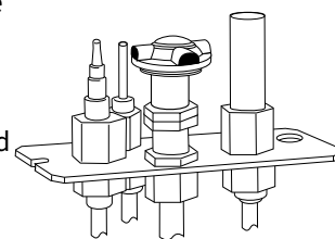
Pilot Assembly
