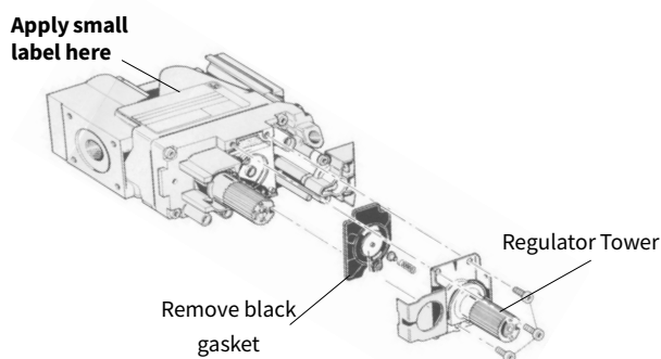
Figure 5.4. Regulator assembly.
