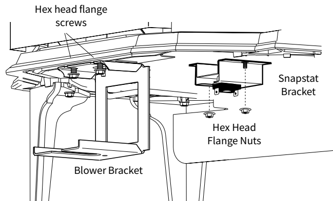
Figure 7.4. Attach Snapstat and Blower Brackets.
