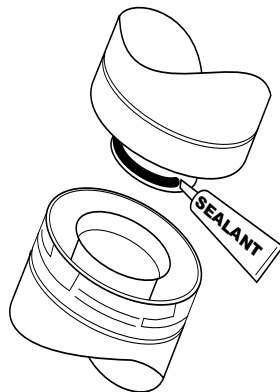
Figure 4.7. DO NOT USE SILICONE SEALANT.
