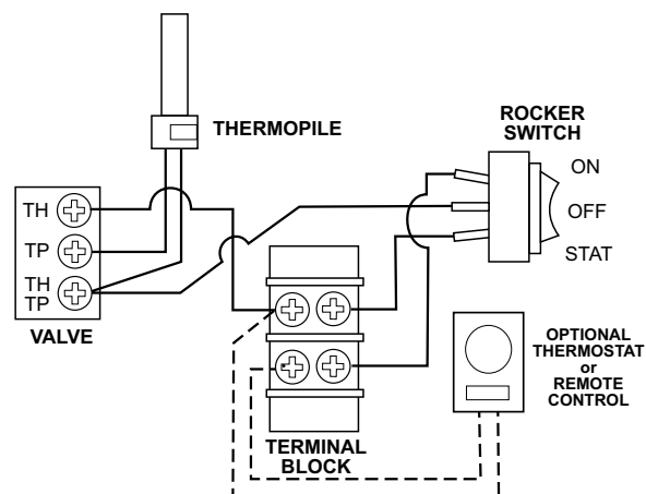
Figure 7.1. Accessory wiring diagram.
