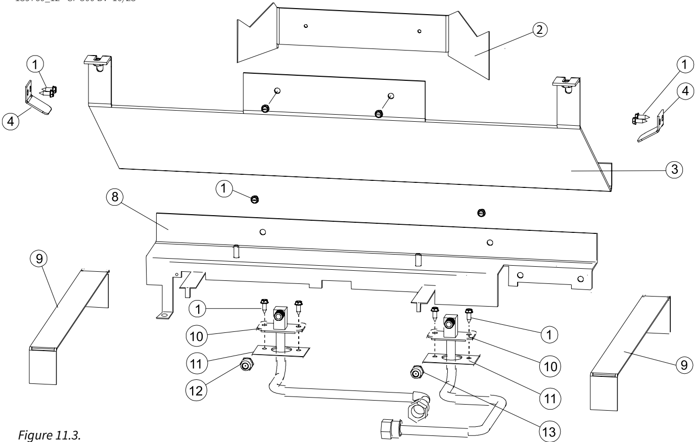
Figure 11.3. GF 500 DV Burner and Pilot components.
