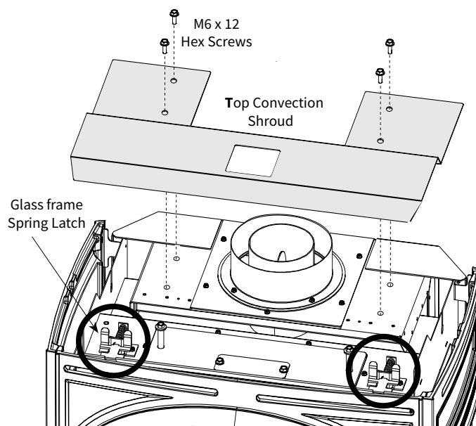
Figure 2.2. Remove the Top Convection Shroud and disengage the glass frame latches.
