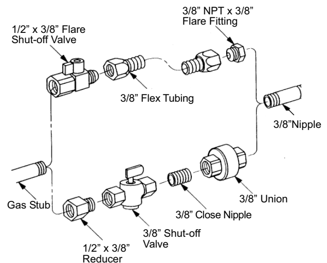
Figure 6.1. Supply valve connection fittings.
