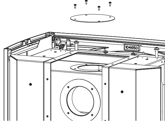
Figure 2.5. Install cover plate over top outlet.
